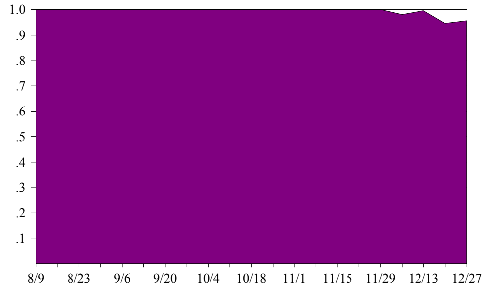
PP Score
